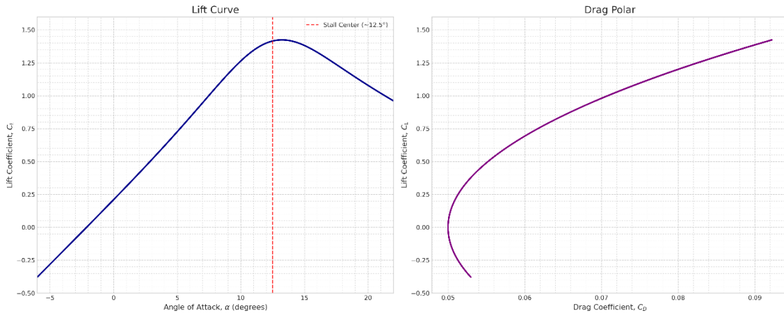
Predicted UAV Aerodynamic Characteristics (NACA 64-212)
